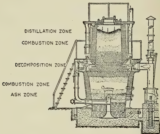
FIG. 96.—Westinghouse Gas-Producer, Type 3.
